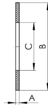
Gasket for flange PN16/40 Flensdichting PN16/40
